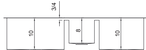
OPENING FOR J-35 DRAIN
