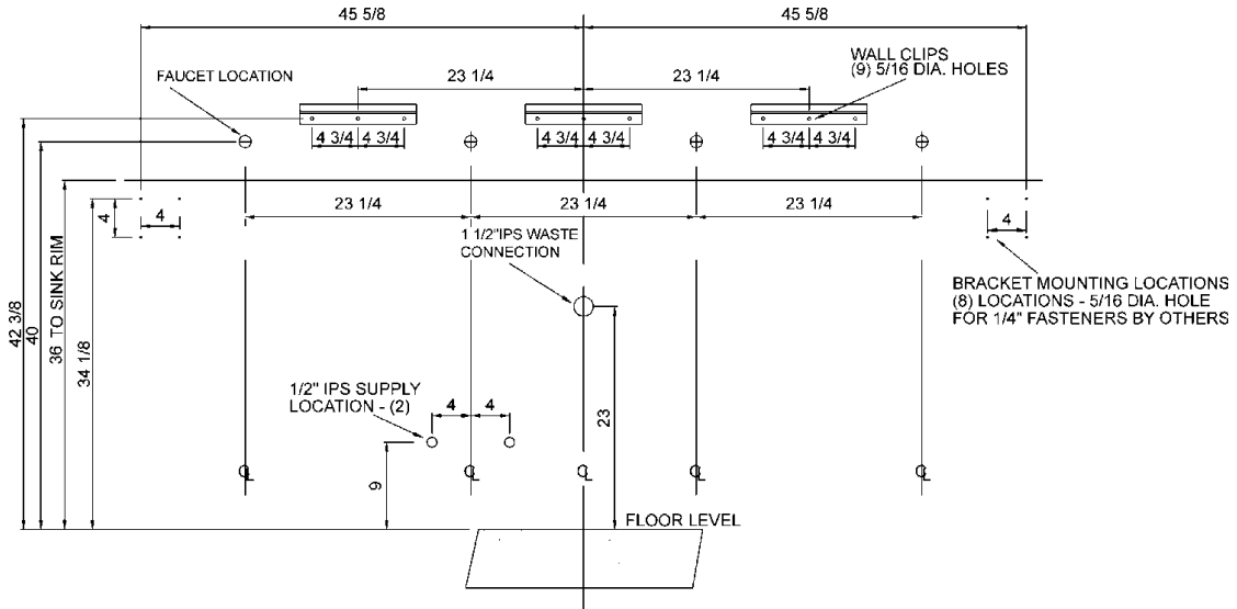
J-9620 ROUGH-IN
