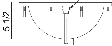
OPENING FOR STANDARD POP-UP DRAIN
