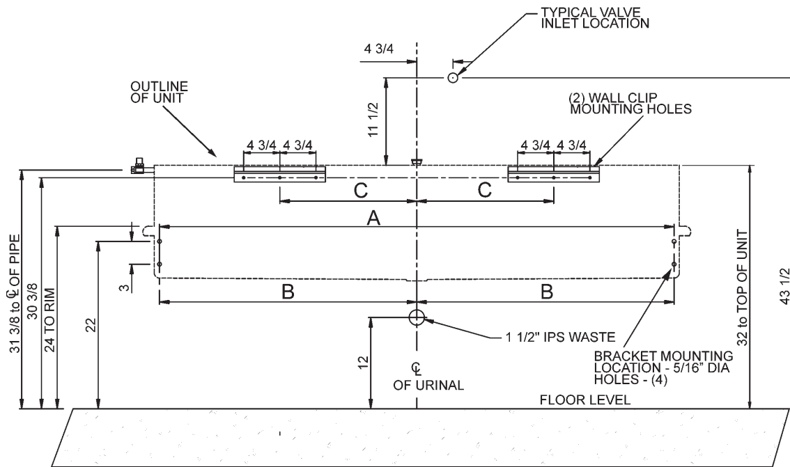
URINAL ROUGH-IN DATA
